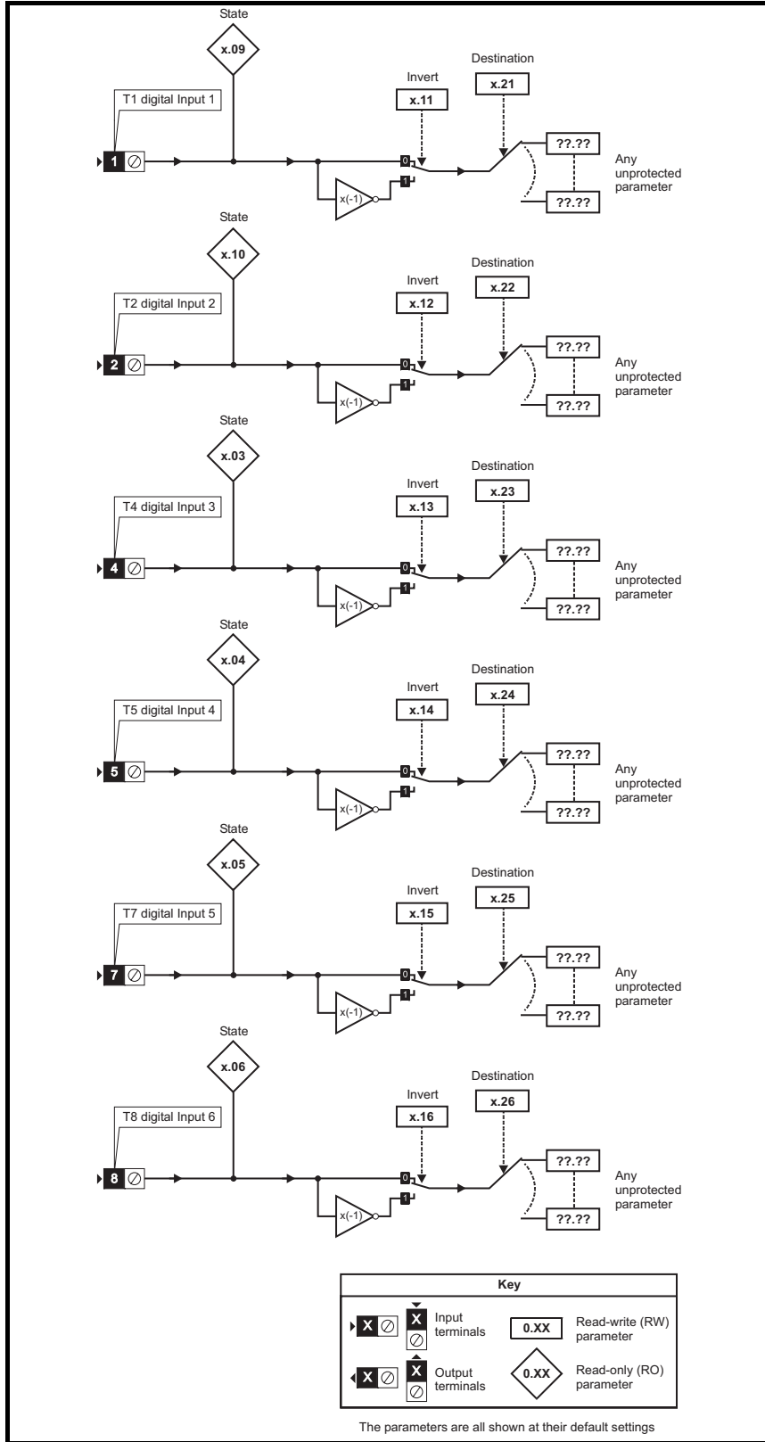
Figure 5-25 Digital input logic diagram
