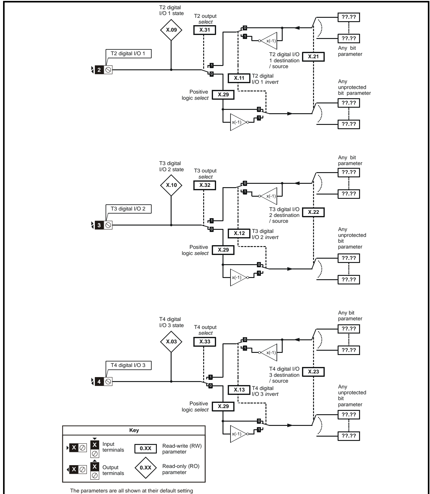
Figure 5-29 SM I/O Plus Digital Input/Output logic diagram 1
