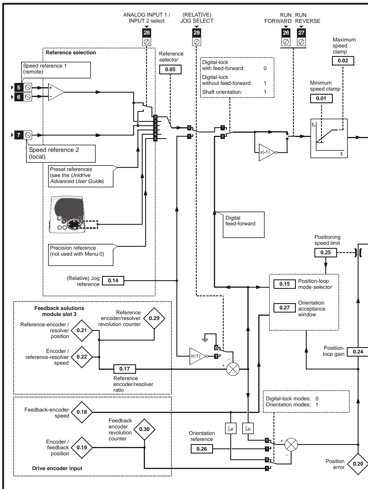
Figure 6-8 Macro 8 Digital lock logic diagram
