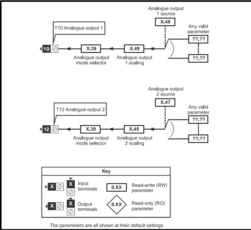
Figure 5-23 Analogue output logic diagram
