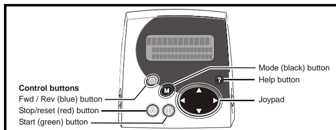
Figure 2-2 SM-Keypad Plus
