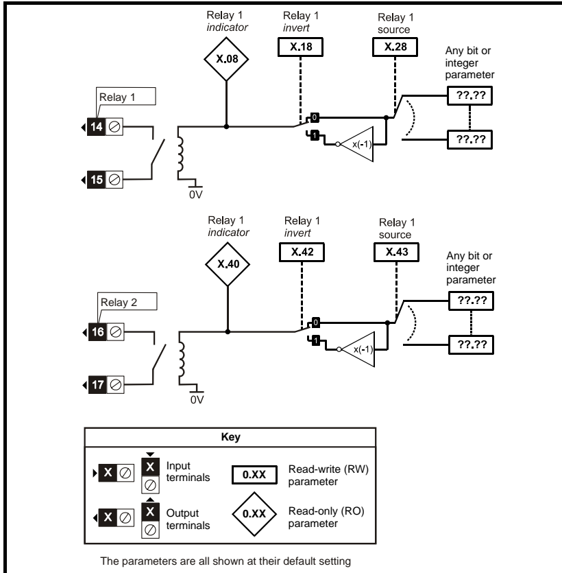
Figure 5-30 Relay logic diagram
