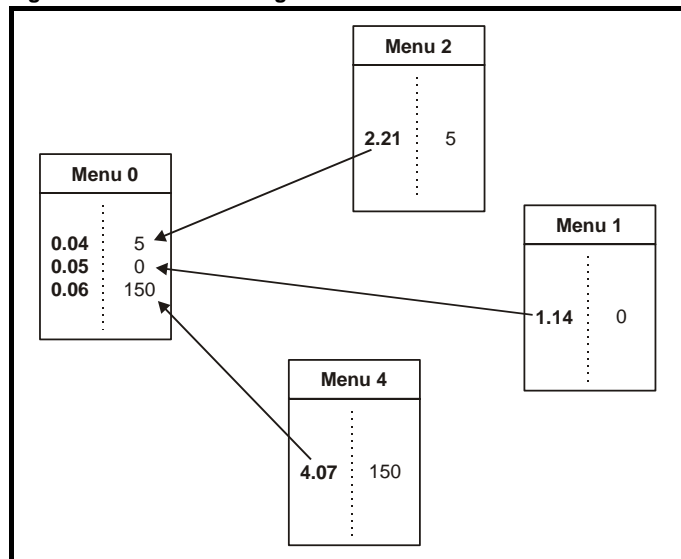
Figure 1-3 Menu 0 cloning
