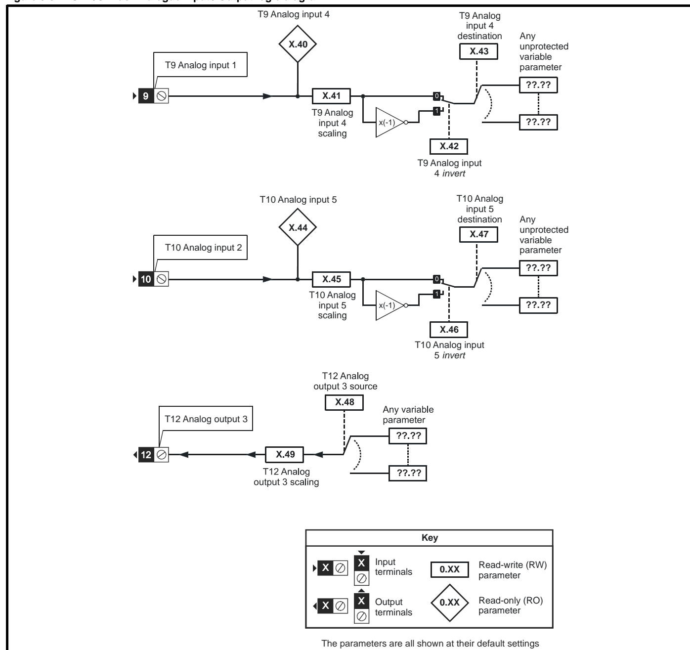
Figure 5-31 SM-I/O Plus Analogue Input / Output logic diagram
