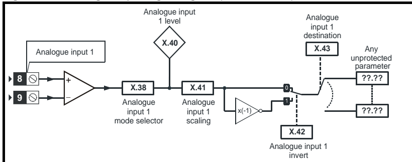
Figure 5-21 Analogue input logic diagram (current mode)
