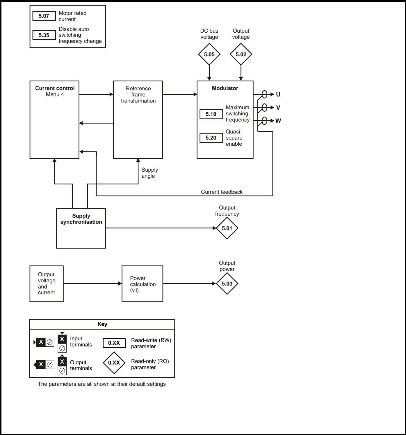
Figure 5-12 Menu 5 Regen logic diagram
