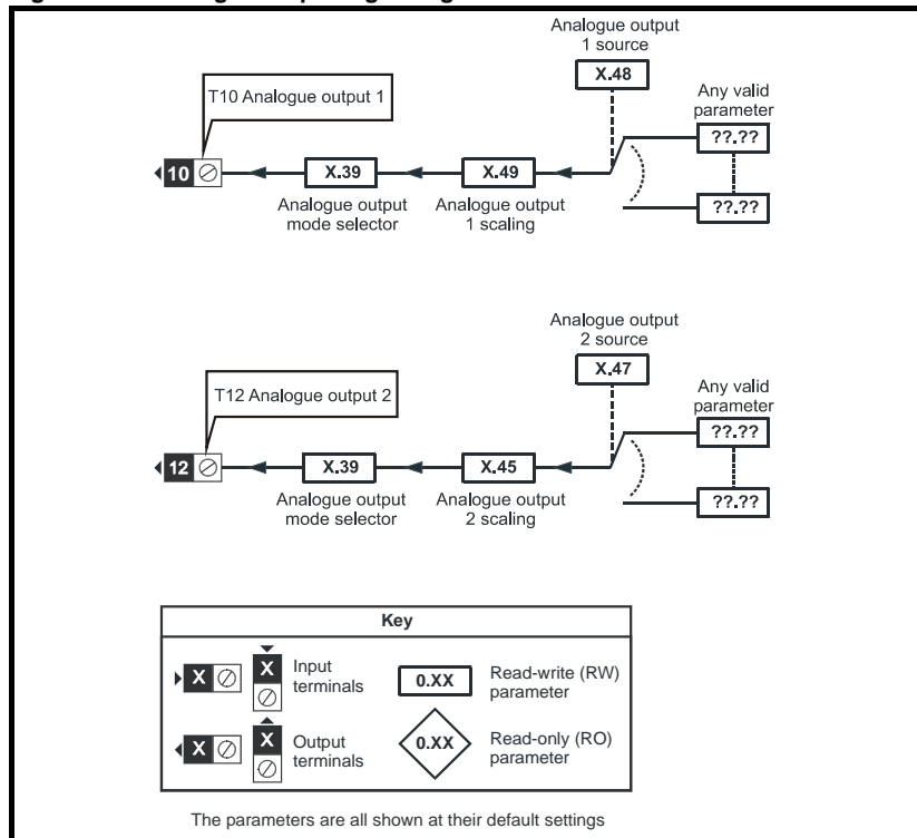
Figure 5-31 Analogue output logic diagram
