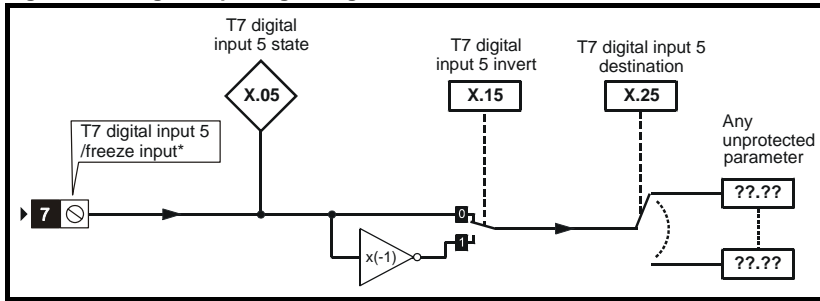
Figure 5-19 Digital input logic diagram
