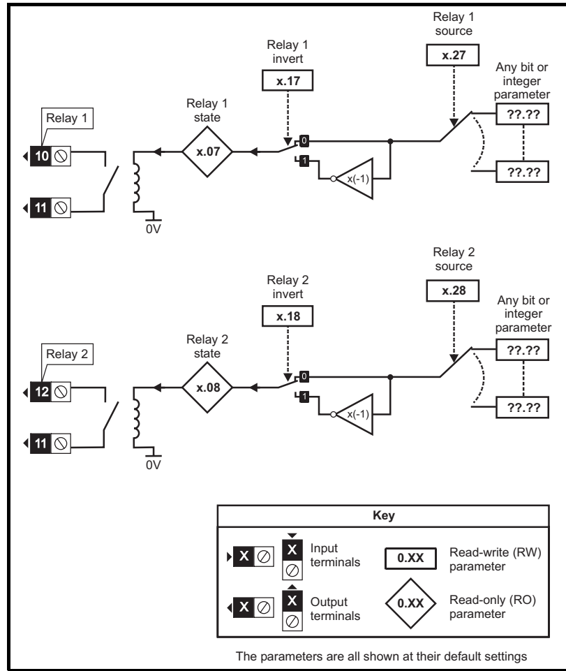
Figure 5-26 Relay logic diagram
