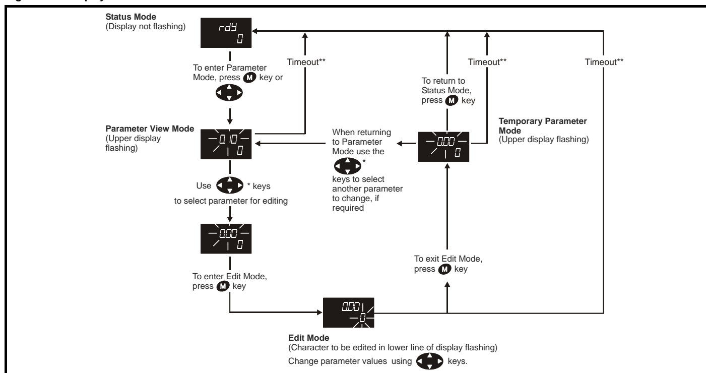
Figure 2-3 Display modes
