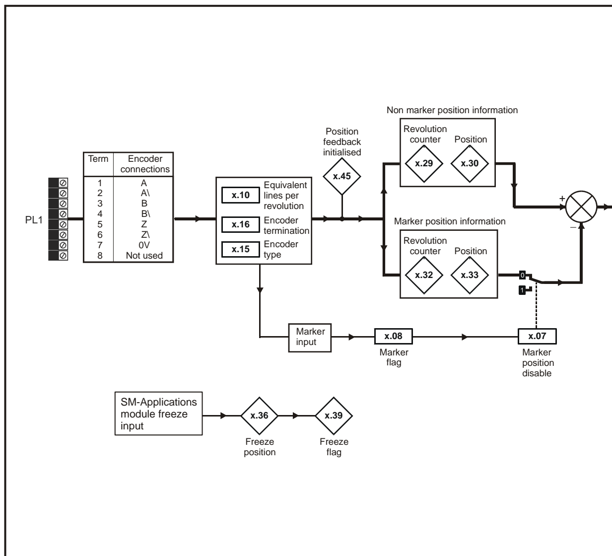
Figure 5-28 SM-Encoder Plus logic diagram
