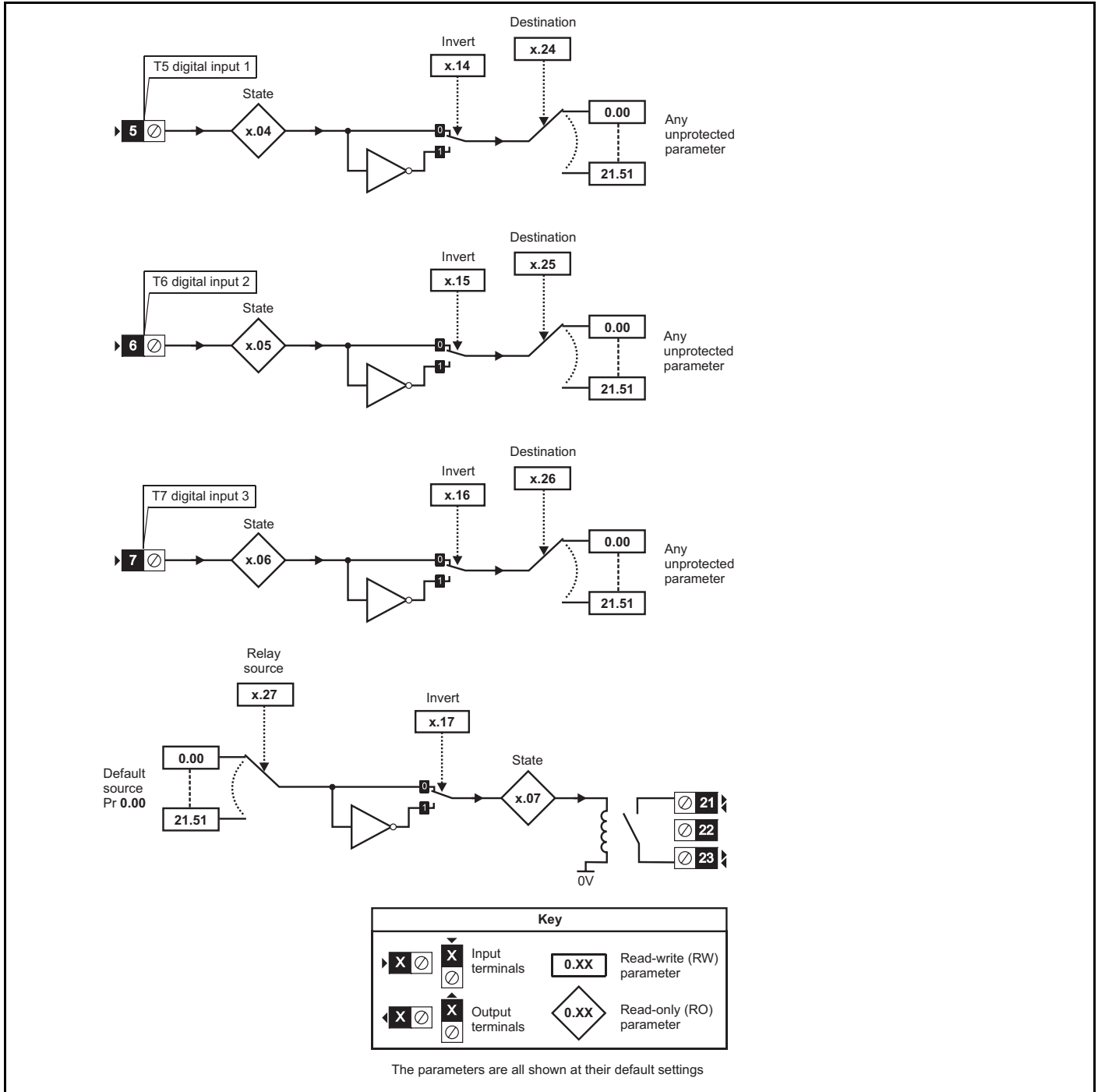
Figure 5-32 SM-I/O Lite & SM-I/O Timer digital I/O logic diagram
