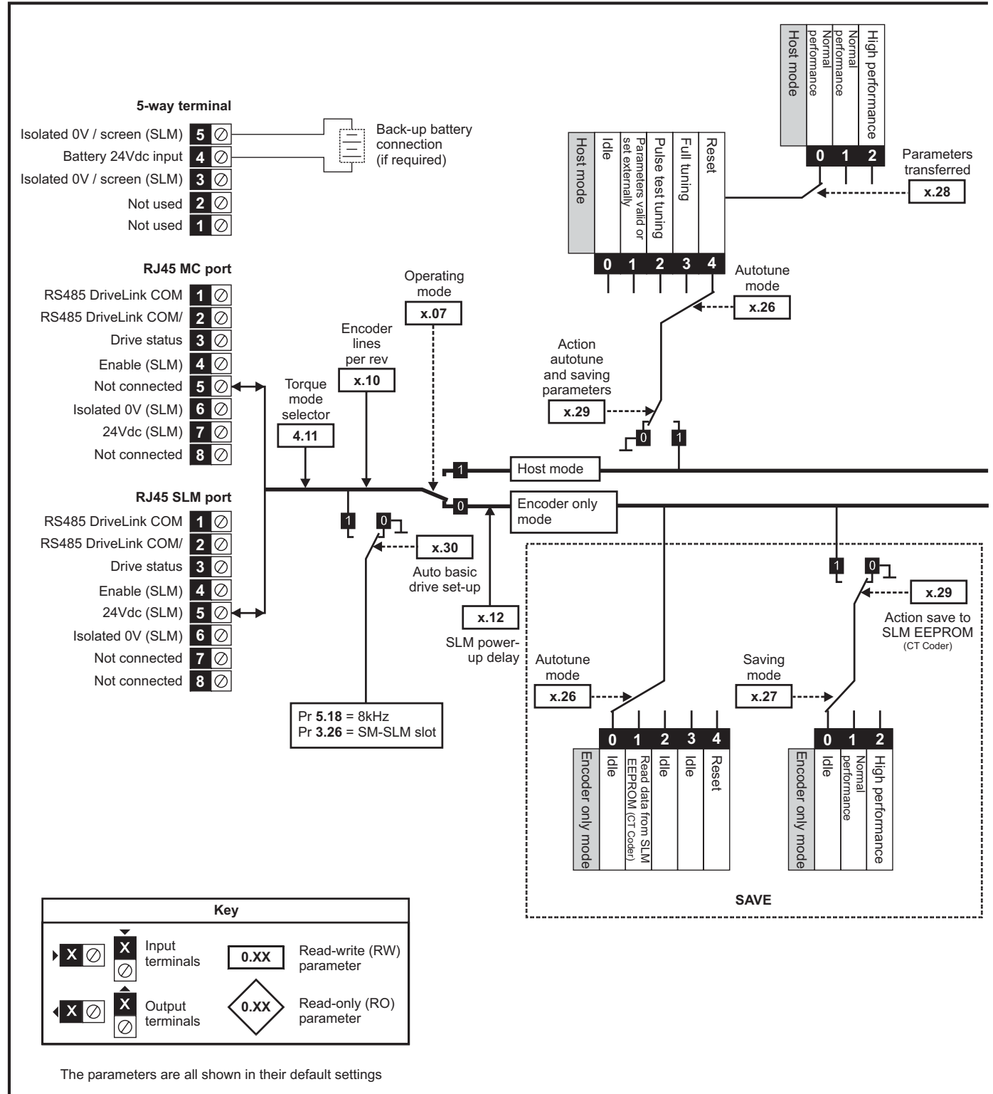
Figure 5-36 SM-SLM logic diagram
