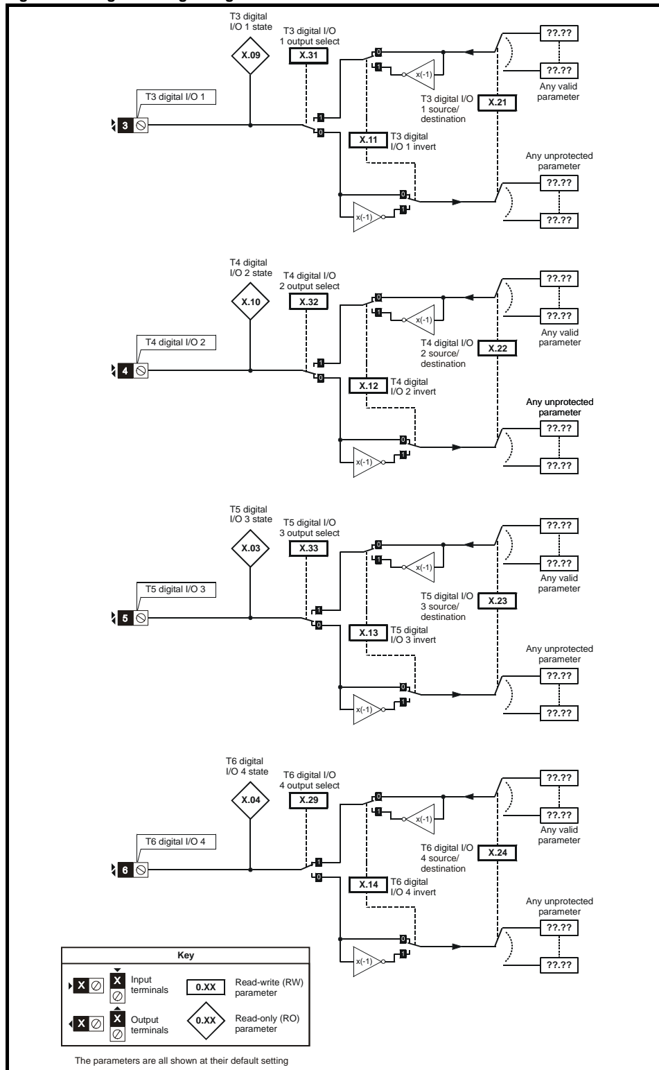
Figure 5-28 Digital I/O logic diagram
