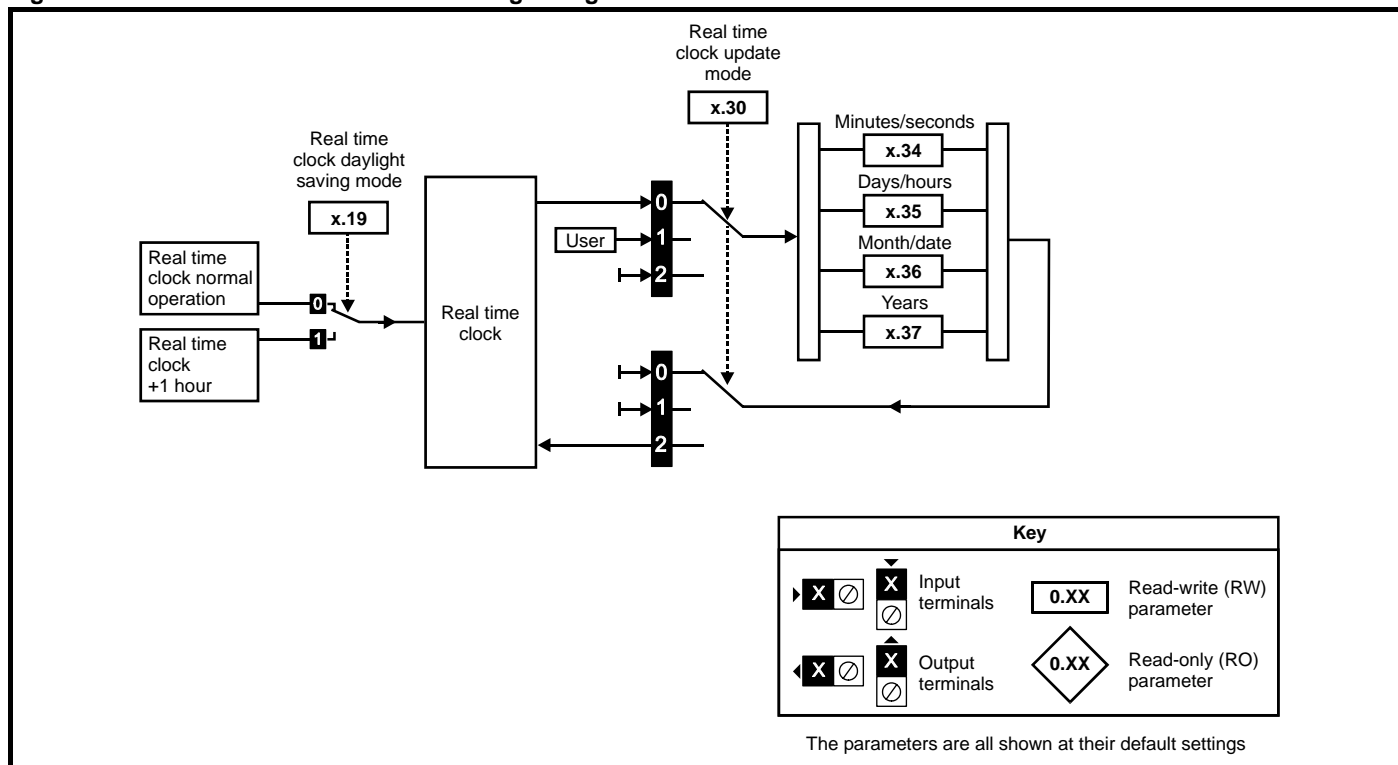
Figure 5-34 SM-I/O Timer real time clock logic diagram
