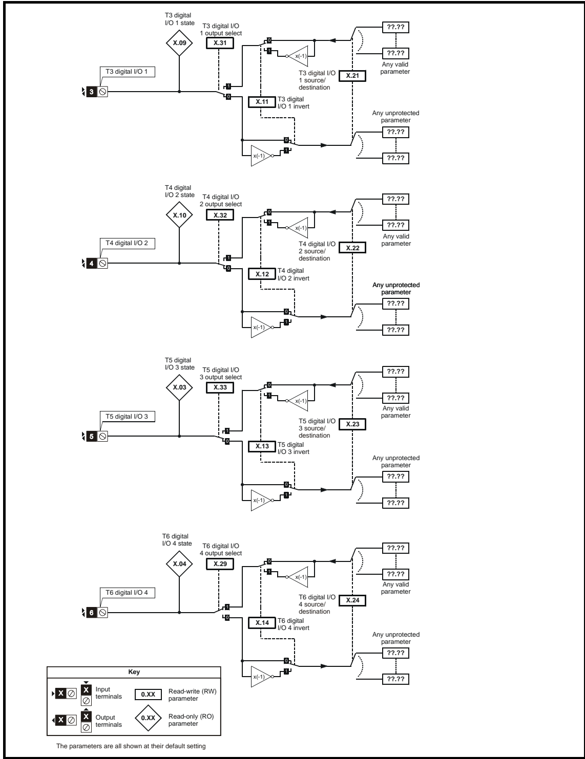
Figure 5-18 Digital I/O logic diagram
