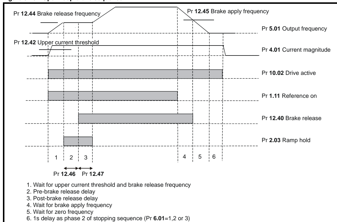
Figure 5-20 Open-loop brake sequence
