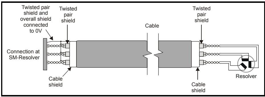
Figure 4-4 Functional shielding requirements
